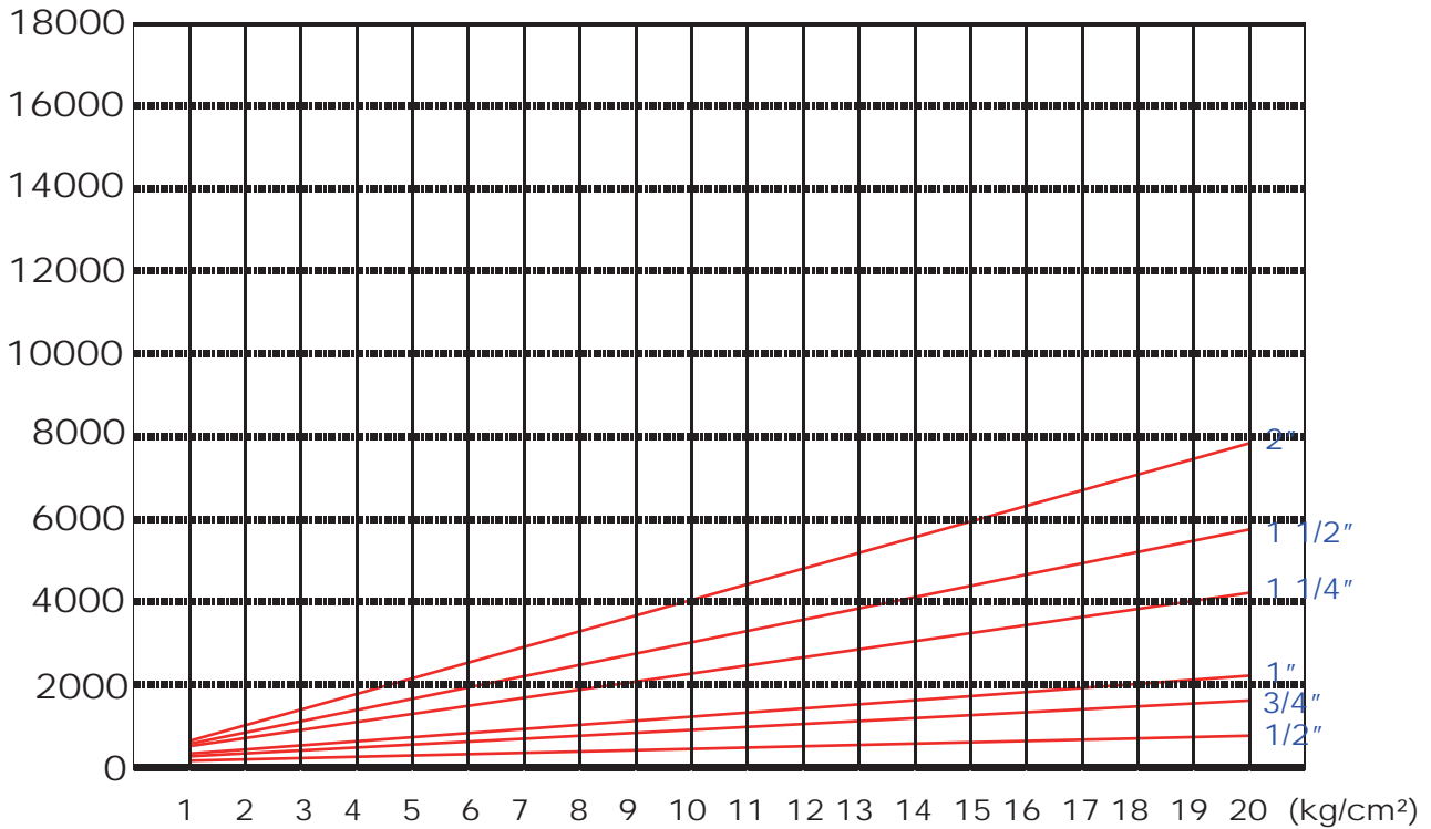
FULL BORE SAFETY VALVE BLOWOUT CAPACITY (kg/h)
