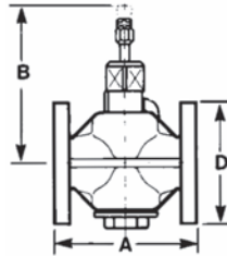
Fig. 401M - Sizes 2" to 4"
